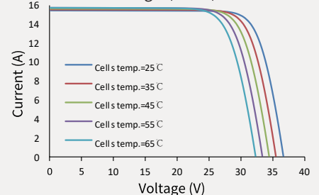
Current-Voltage (460W)
